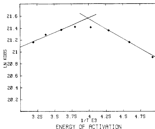
Figure 1. \ln k_{\text{obsd}} (s -1 ) vs. 1/T (K -1 × 1000) for the addition of p -CF 3 C 6 H 4 CBr to tetramethylethylene. The left-hand portion of the correlation (312–263 K) leads to E_a = -1 kcal/mol. The right-hand correlation (232–203 K) leads to E_a = 1.3 kcal/mol. See text for discussion.
